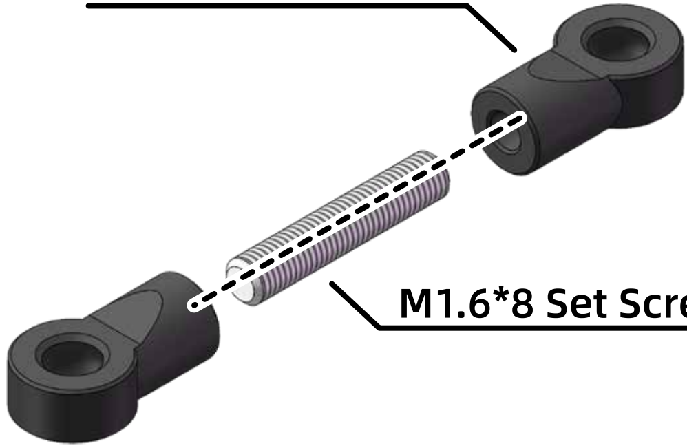
Short Ball End Cap
