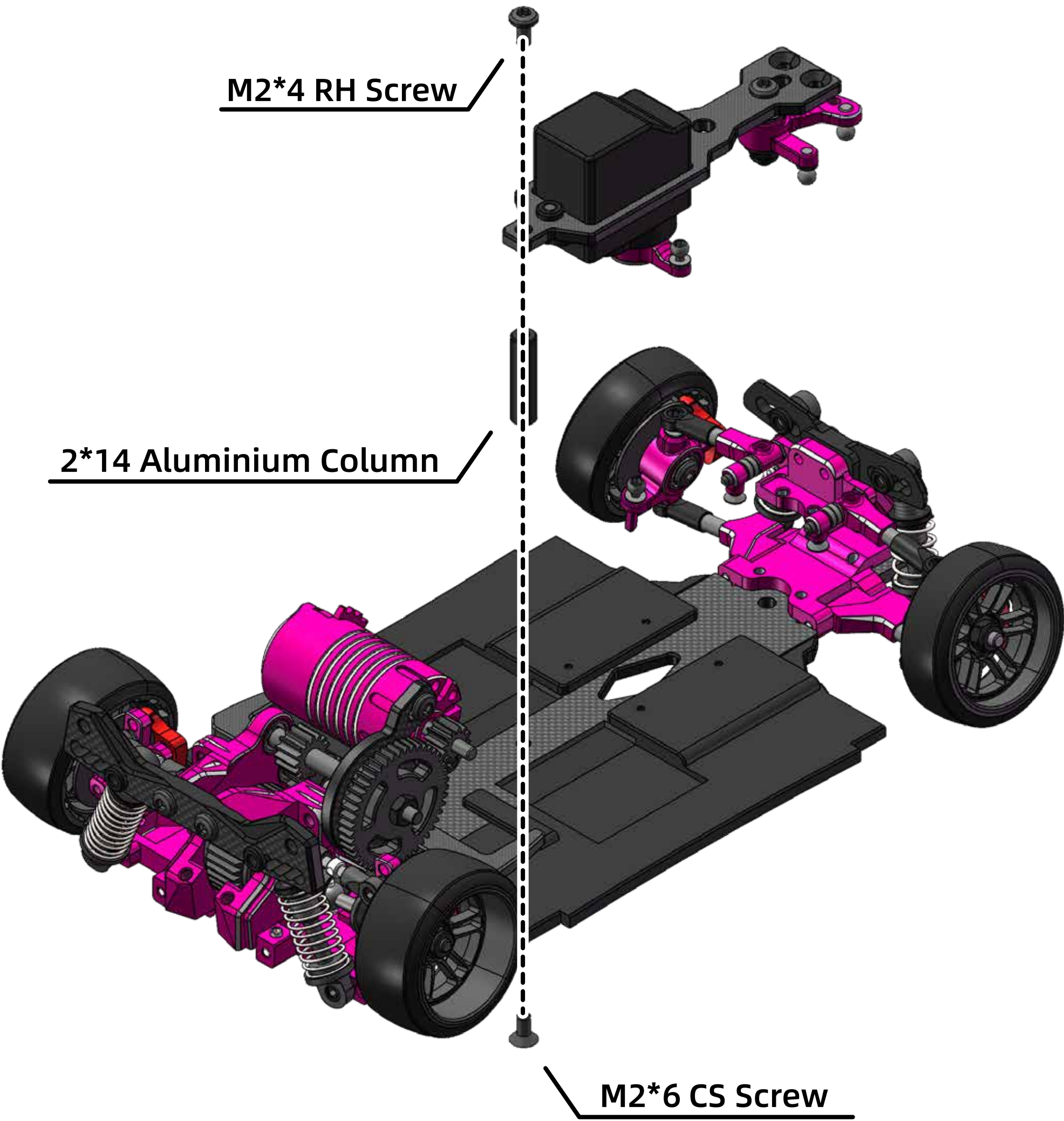
2*14 Aluminium Column x 1
