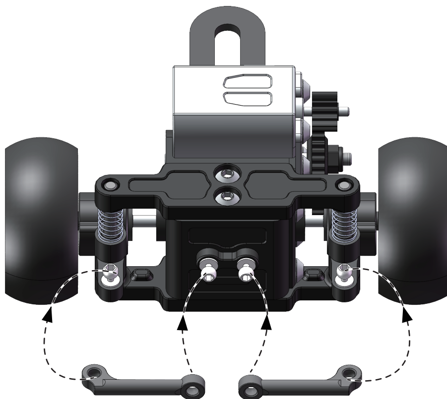
Short Rear Tie Rod
