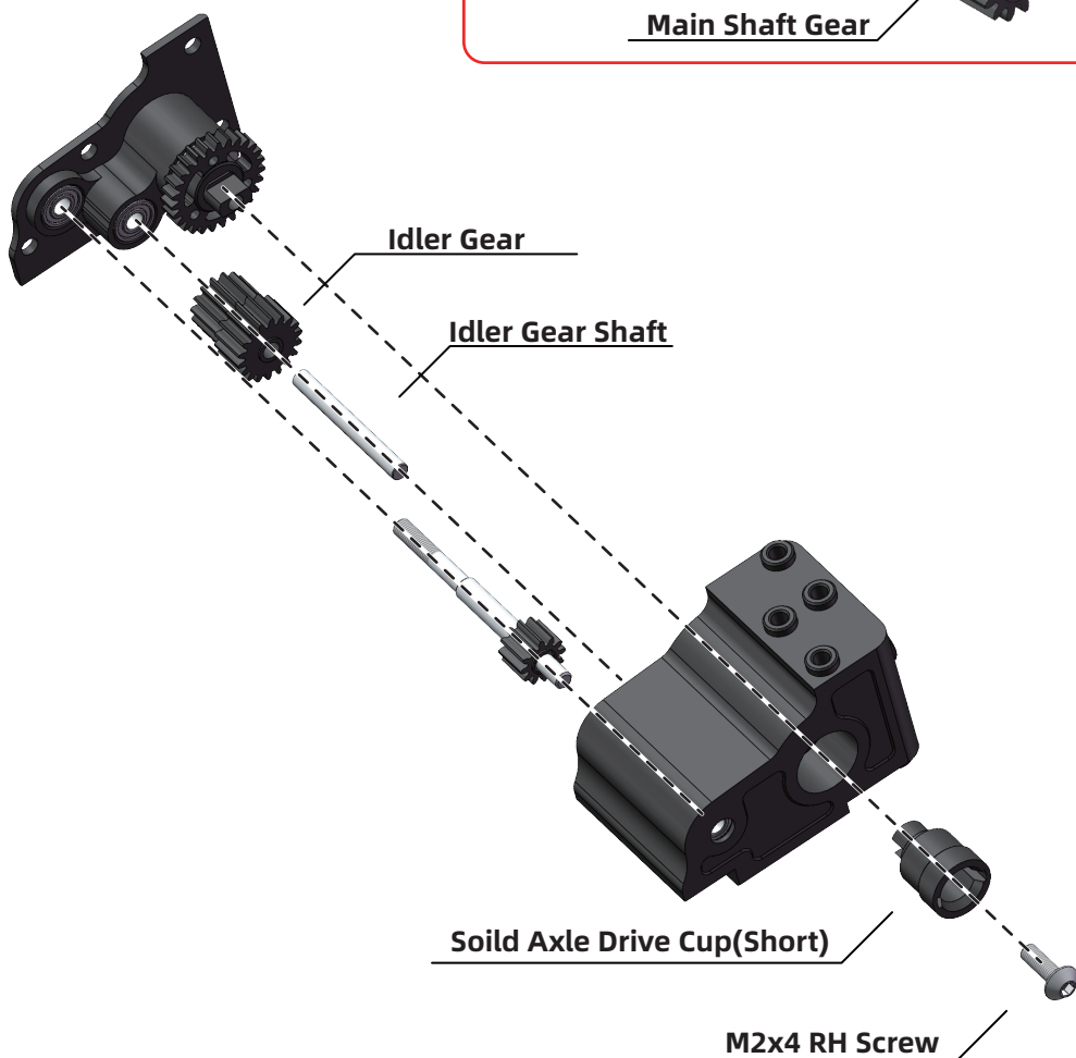
直轴接杯 短 Solid Axle Drive Cup(Short) x 1
