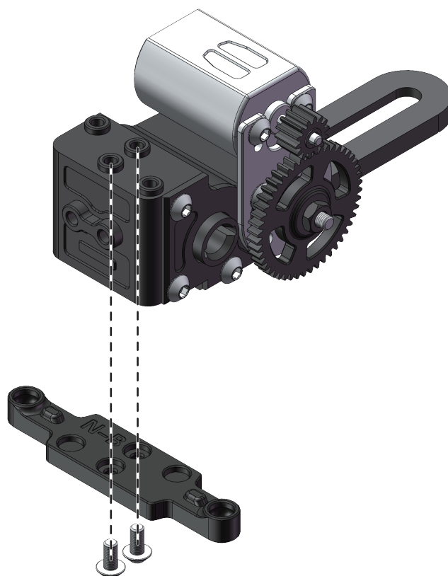
M2x3 RH Screw
