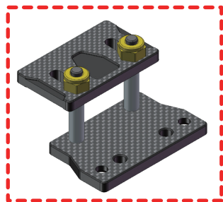
可调车舌 Adjustment Front Body Mount
