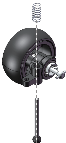
M2x3 RH Screw
